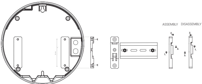
Figure No.8: Assembly on DIN rail
